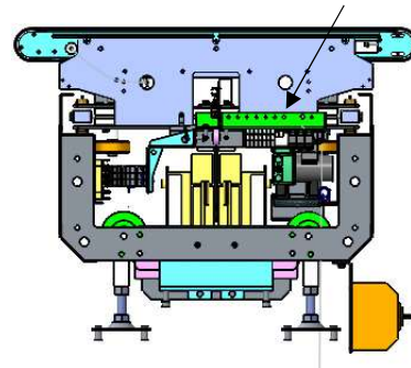
Leaky wave cable position
